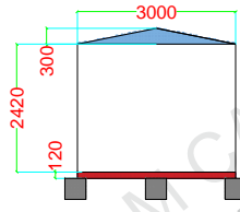
Left Elevation
