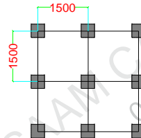
Foundation SKID Plan Precast block 40 x 40 x 40
