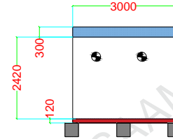
Back Elevation
