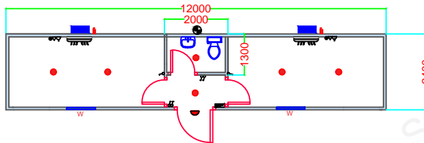
FLOOR PLAN
