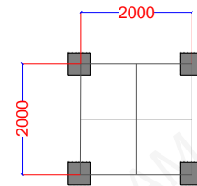
FOUNDATION PLAN PRECAST BLOCK SIZE 40 X 40 X 40
