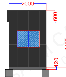
LEFT ELEVATION
