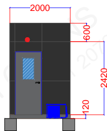
BACK SIDE ELEVATION
