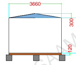
RIGHT SIDE ELEVATION
