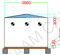
BACK ELEVATION
