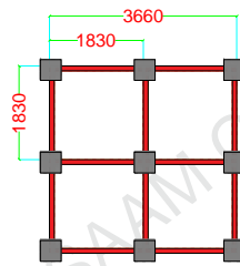
SKID PLAN | FOUNDATION PLAN PRECAST BLOCK SIZE 40 X 40 X 40
