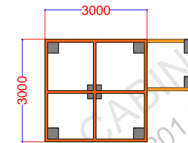
FOUNDATION PLAN PRECAST BLOCK SIZE 40 X 40 X 40
